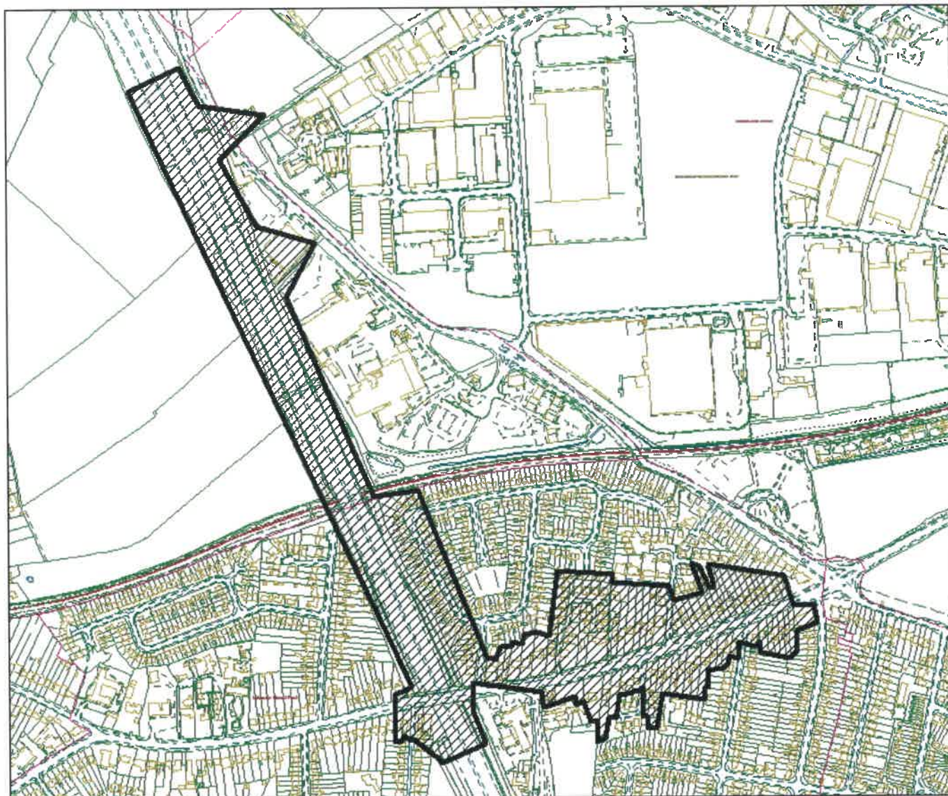
Figure 2: Map of AQMA 3 – M1 corridor between Thorpe Astley and Leicester Forest East. Black border and shading denotes extent of AQMA.
